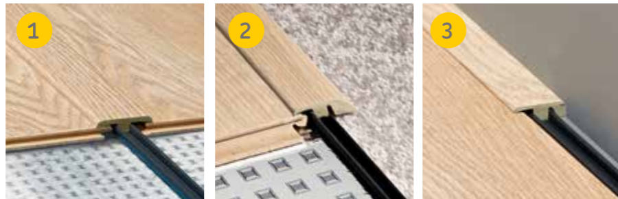
1 Expansion Profile 1850 x 33.4 x 10.5 mm 2 Adaptor Profile 1850 x 43.7 x 12.5 mm 3 Edge Profile 1850 x 33.4 x 12.5 mm
