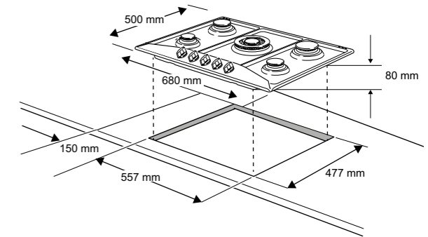
5 BURNER GAS HOB
