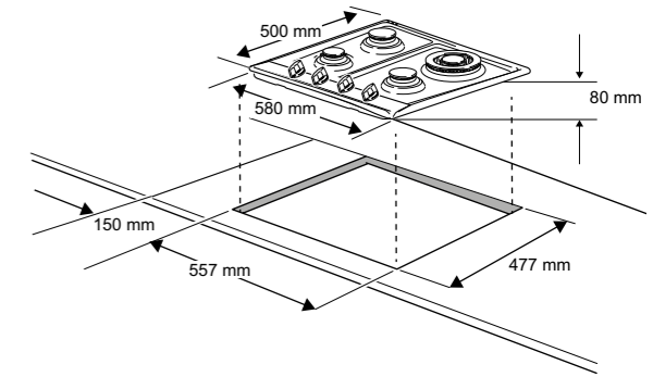
4 BURNER GAS HOB
