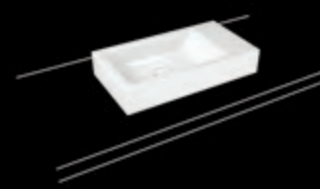
CONO Countertop handbasin Tap hole can be positioned on right or left Model No. 3074 / L 55cm x W 30cm x H 10cm
