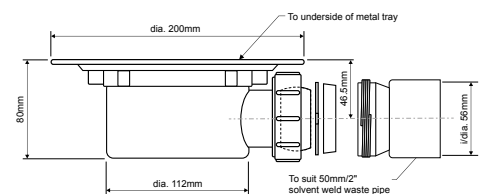
Standard waste option for tiled floors
