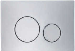
Rondo dual flush push plate 210(w) x 137mm(h) Chrome TR9012
