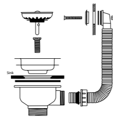
SQUARE OVERFLOW WASTE KIT CPK1501
