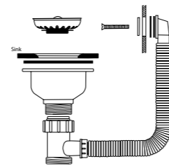
SQUARE OVERFLOW WASTE KIT CPK1900 - Chrome CPK2500 - Brushed steel
