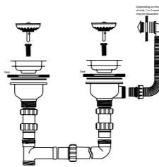
WASTE AND BOWL CONNECTION KIT CPK801
