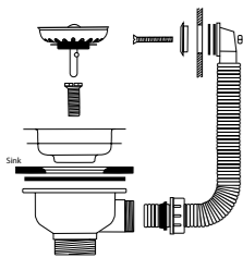
ROUND OVERFLOW WASTE KIT CPK501
